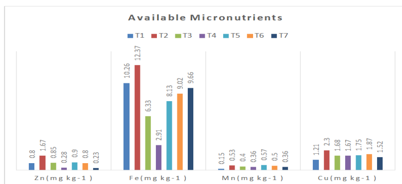
Fig. 2. Effect of various cropping systems on Soil Available Micronutrients
