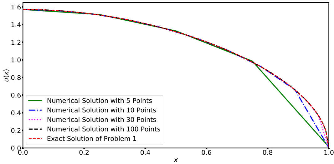
Fig. 1. Plot of exact solution and numerical solution for problem 1
