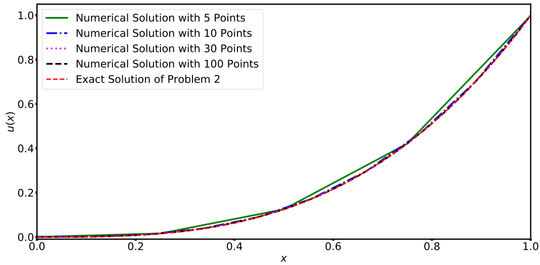
Fig. 2. Plot of exact solution and numerical solution for problem 2
