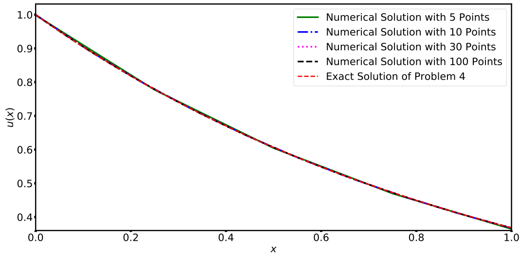
Fig. 4. Plot of exact solution and numerical solution for problem 4
