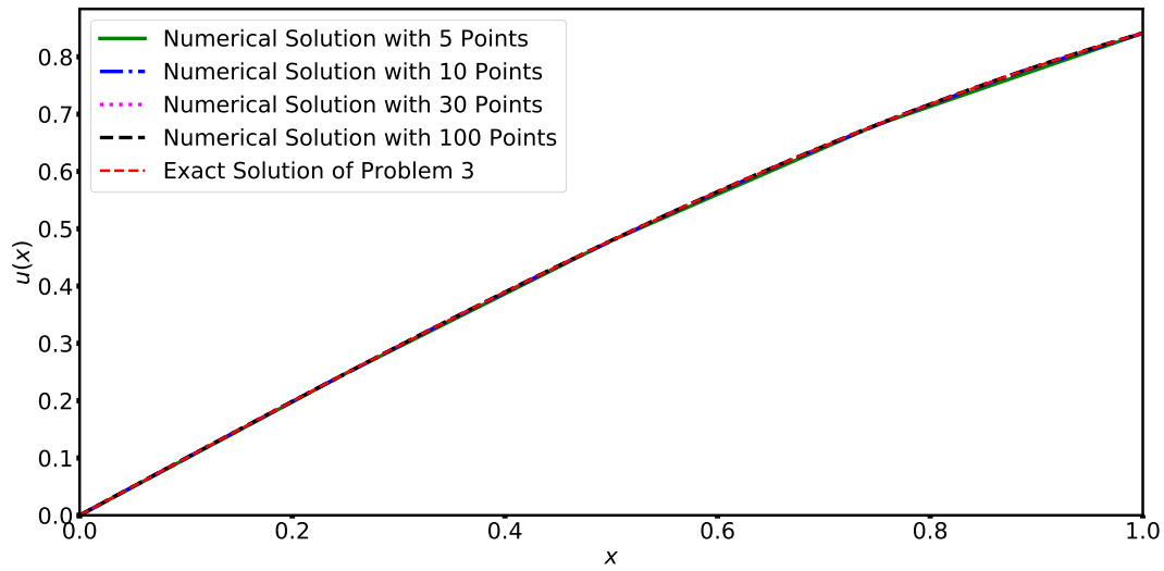
Fig. 3. Plot of Exact solution and numerical solution for problem 3
