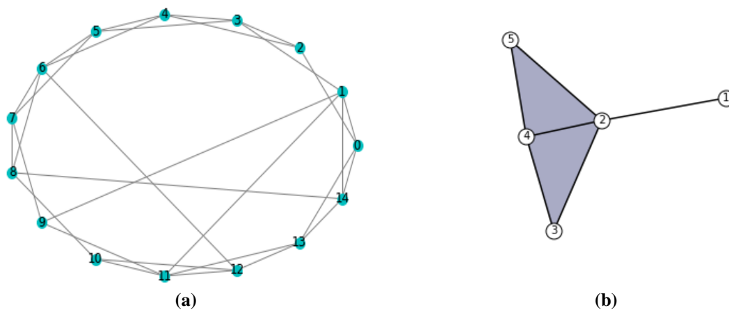
Fig. 3. Two types of network structure diagram (a) Random network. (b) Higher-order network
