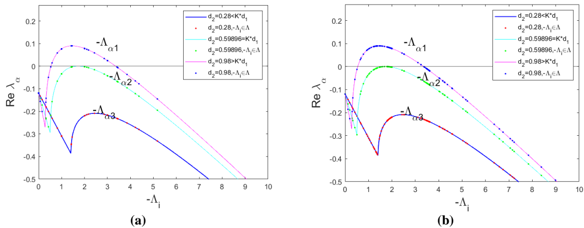
Fig. 4. The eigenvalues distribution of system (1). (a) and (b) represent the eigenvalues distribution of system (1) in the random network and higher-order network, respectively
