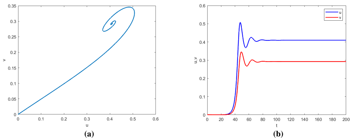
Fig. 2. (a) The phase diagram in Eq (1). (b) The time series diagram of u and v
