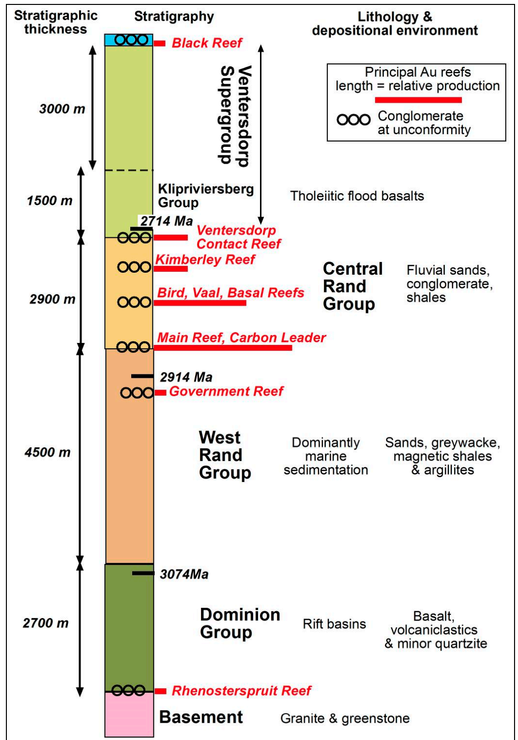
Figure 3. Stratigraphic column showing approximate thickness of various Archean successor basins with their main rocks and reef groups. The red bars for the major gold reef groups show their relative productions. The Dominion, West Rand Group, and Black Reef production bars are approximate only, based on various sources. The OOO symbol denotes reef packages.
