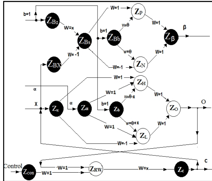
Fig. 5. CAM cell with \beta
