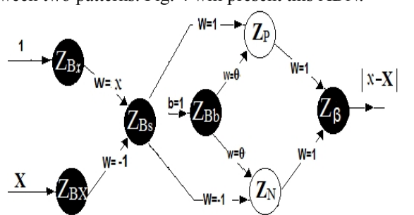
Fig. 4. Absolute Distance Network
