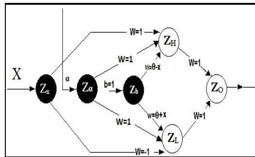
Fig. 2. Exclusive X gate with \alpha
