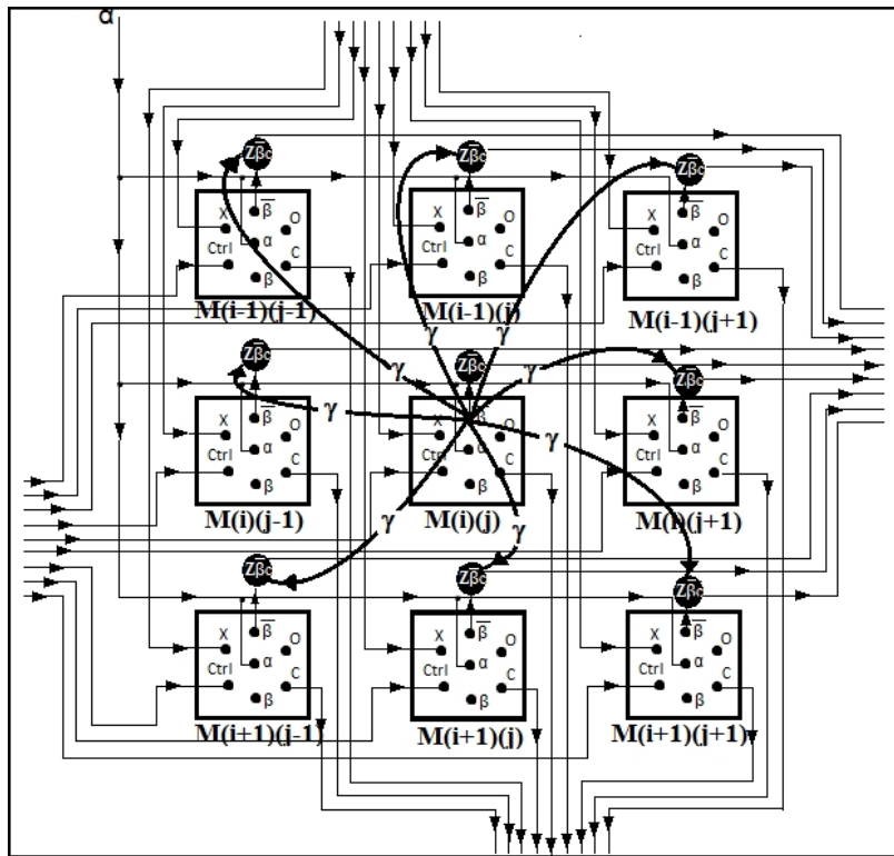
Fig. 9. First order \bar{\beta} sharing
