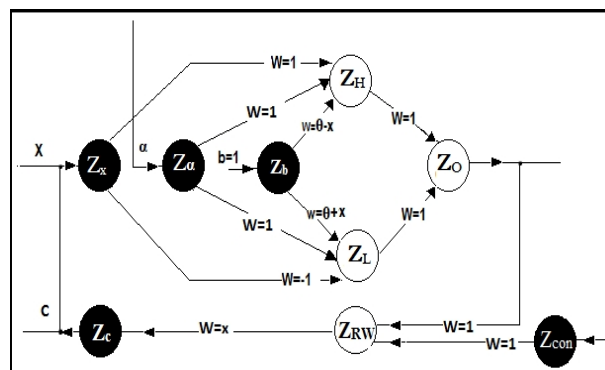
Fig. 3. CAM cell with \alpha
