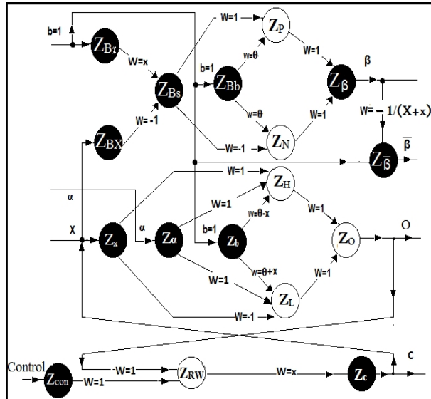
Fig. 6. CAM Cell with \bar{\beta}
