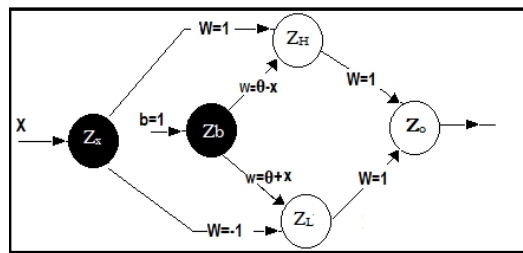
Fig. 1. Exclusive X gate
