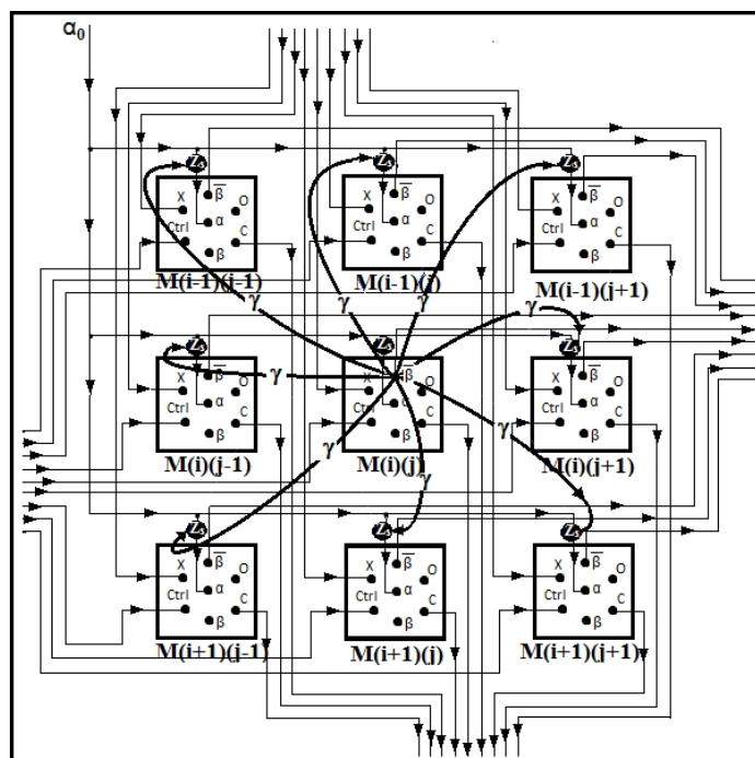
Fig. 10. First order \alpha sharing
