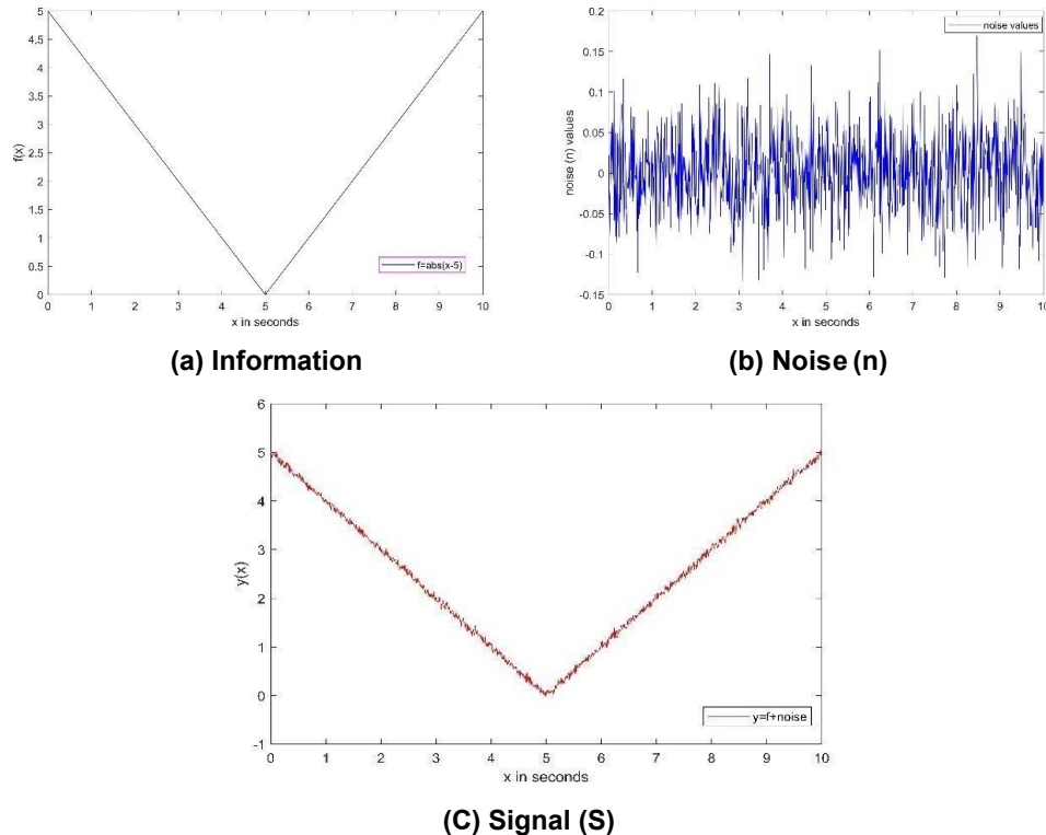
Fig. 1. Graphs depicting the general system in equation 2.1
