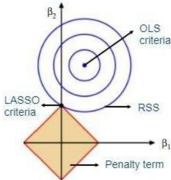
Fig. 16. Geometric representation of LASSO regression [22]
