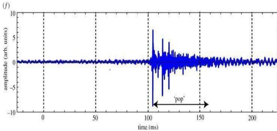
Fig. 9. A graph showing the generation of pop (burst) noise
