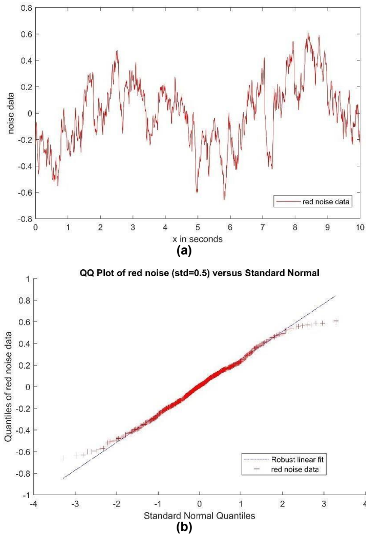
Fig. 14. Representation of Brownian/red noise and its quantile-quantile plot
