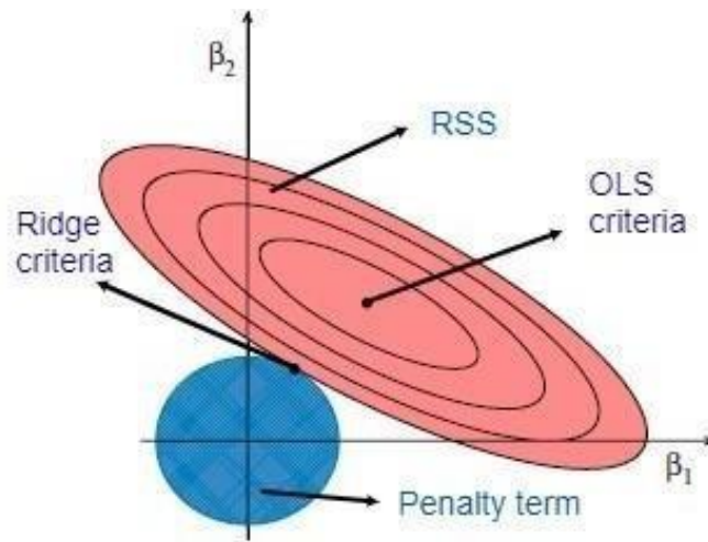
Fig. 15. Geometric representation of ridge regression [19]
