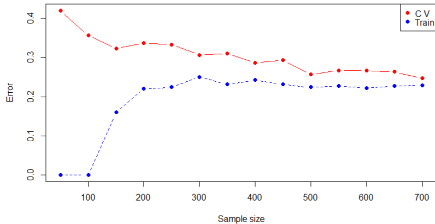
Fig. 8. Train errors Vs Test errors plot for the logistic model
